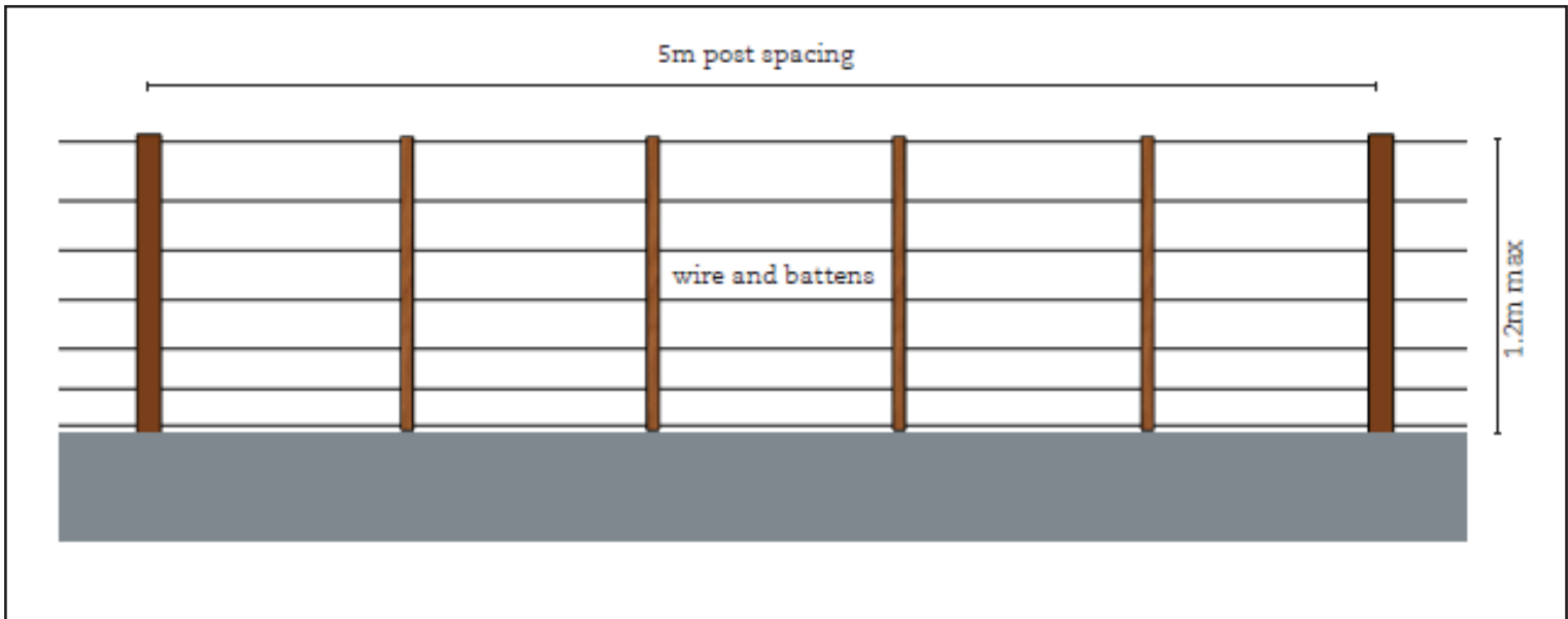
Figure 11 - Fencing Detail 1 - Maunga Edge Road
